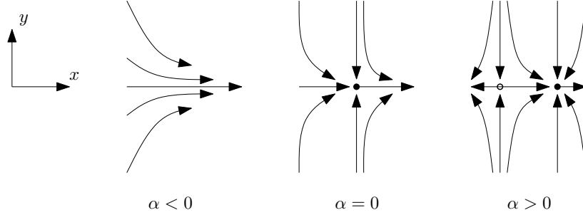
Figure 2.1: Phase portraits for (2.1.2)
