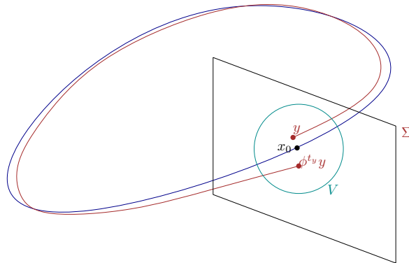
Figure 2.5: Poincaré Map Illustration
